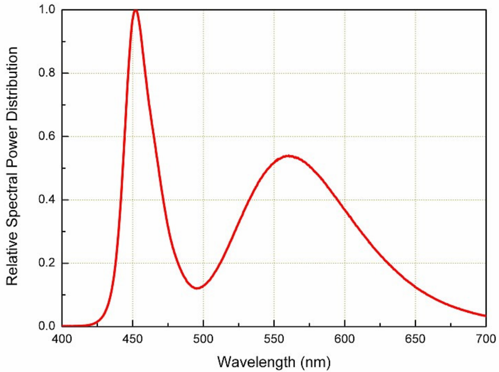
For Cool-White, @ Thermal Pad Temperature = 25°C
