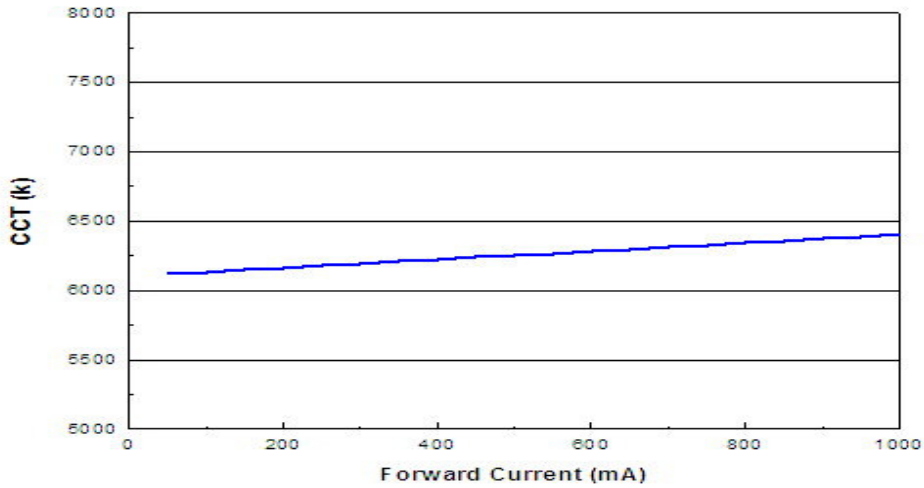
For Cool-White @ Thermal Pad Temperature = 25°C
