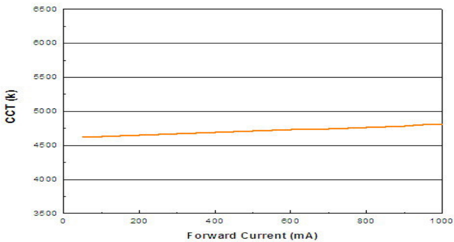
For Neutral-White @ Thermal Pad Temperature = 25°C
