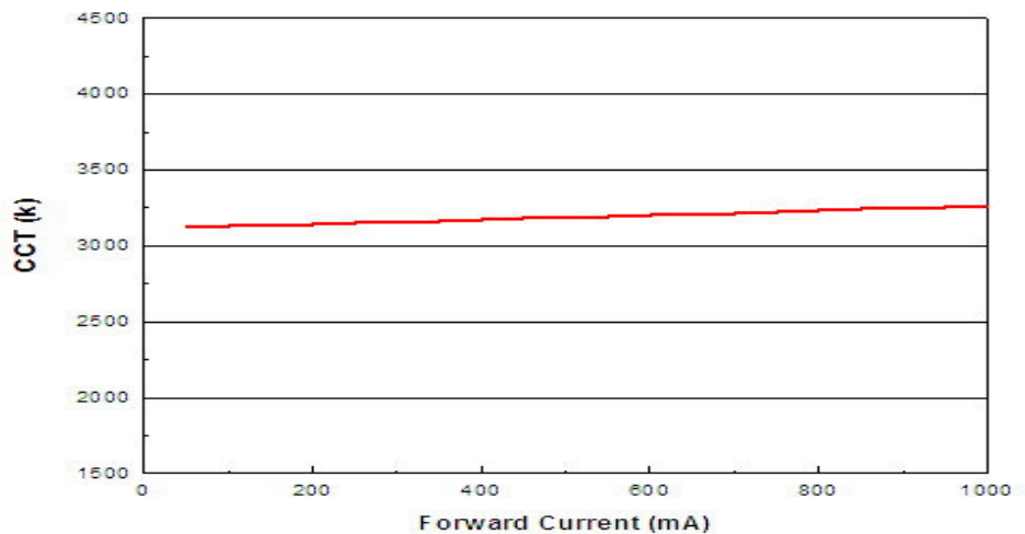
For Warm-White @ Thermal Pad Temperature = 25°C
